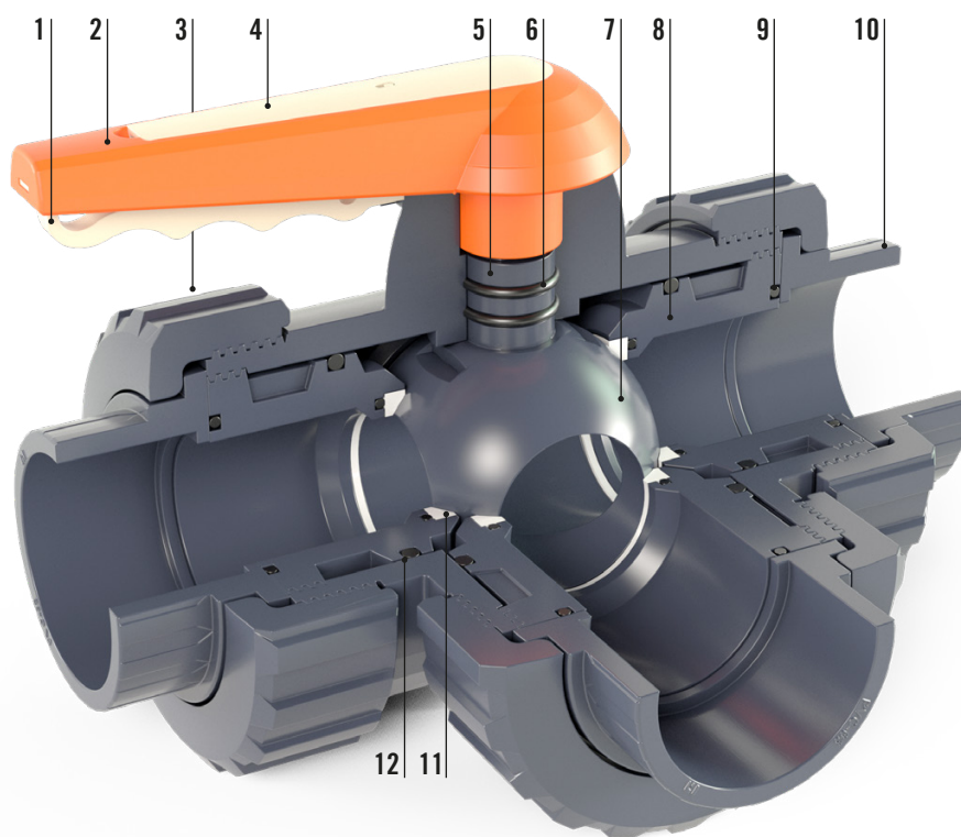
MODELO "T" / "T" MODEL
